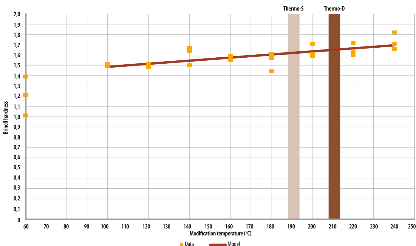
Figure 24. The impact of thermal modification (3 h) on Brinell hardness of pine (source: VTT).
