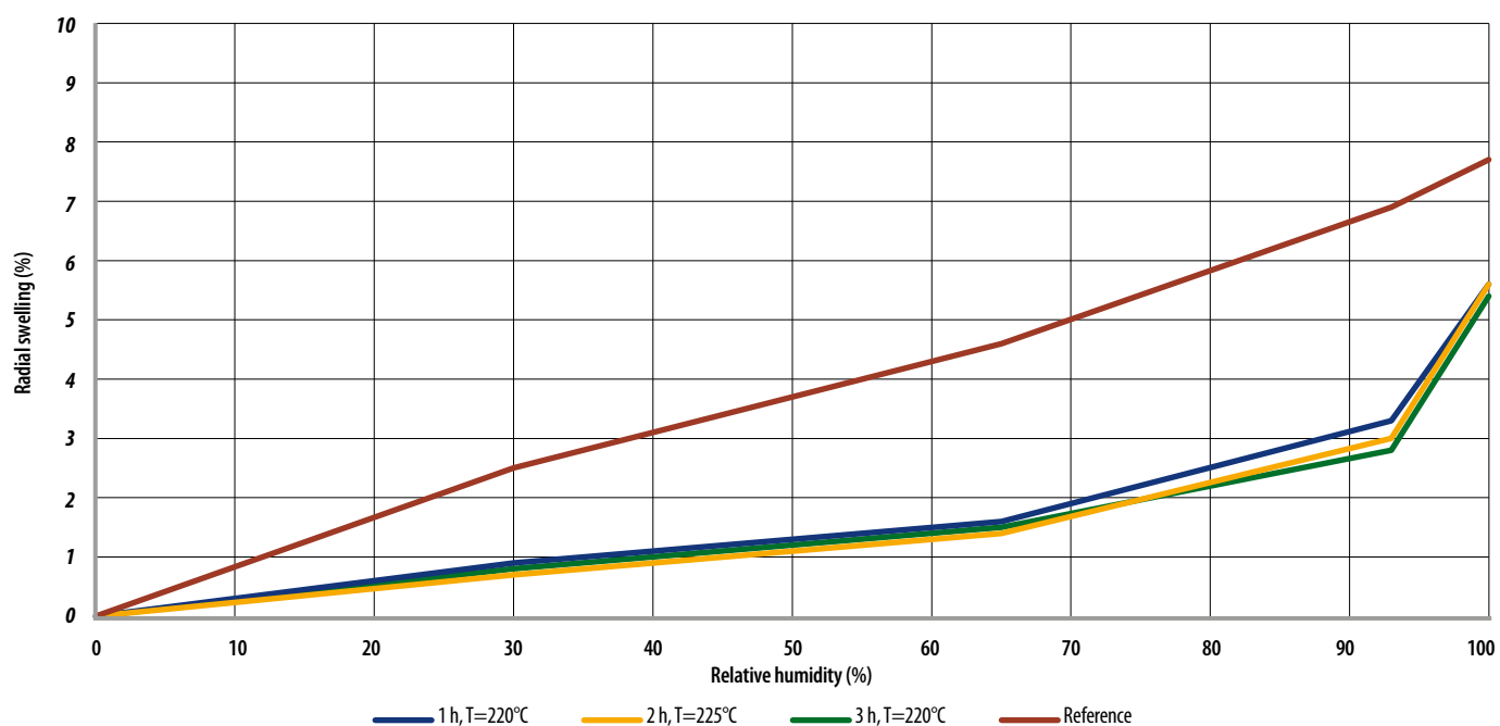
Figure 27. Radial swelling of spruce as a function of relative humidity (source: VTT).
