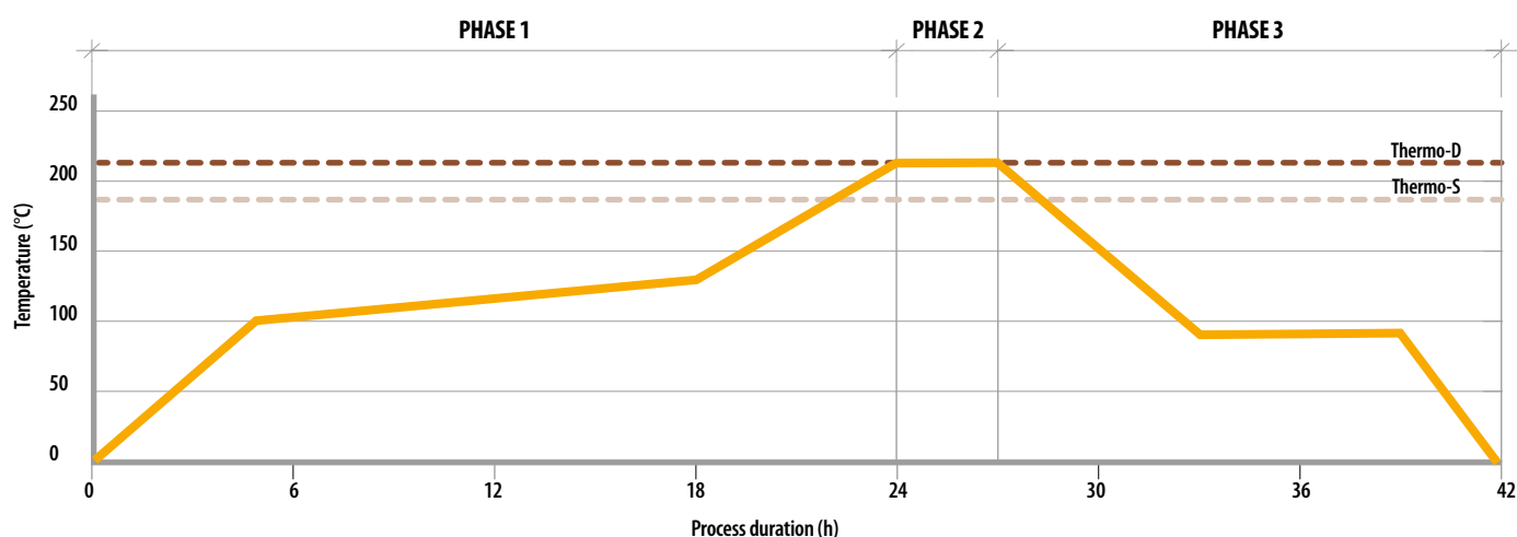
Figure 3. An example of the ThermoWood® process for Nordic softwood (product class Thermo-D).
